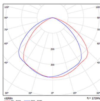
High Bay HPI 400W
