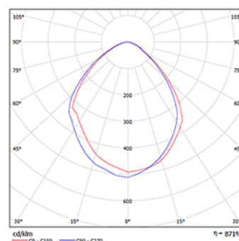
High Bay HPI 250W
